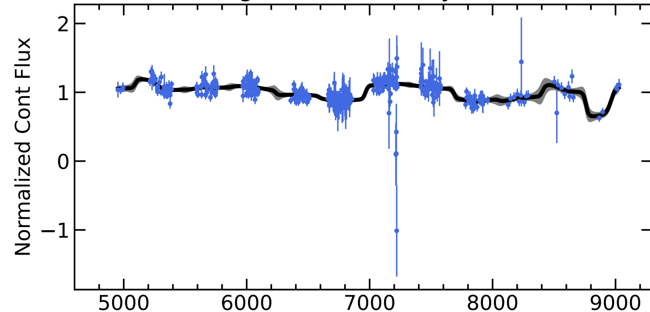
RM000 Light Curves (w/ PyROA model)
