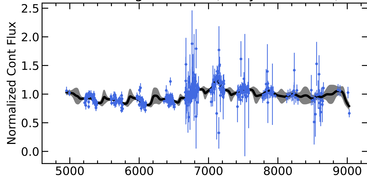
RM001 Light Curves (w/ PyROA model)
