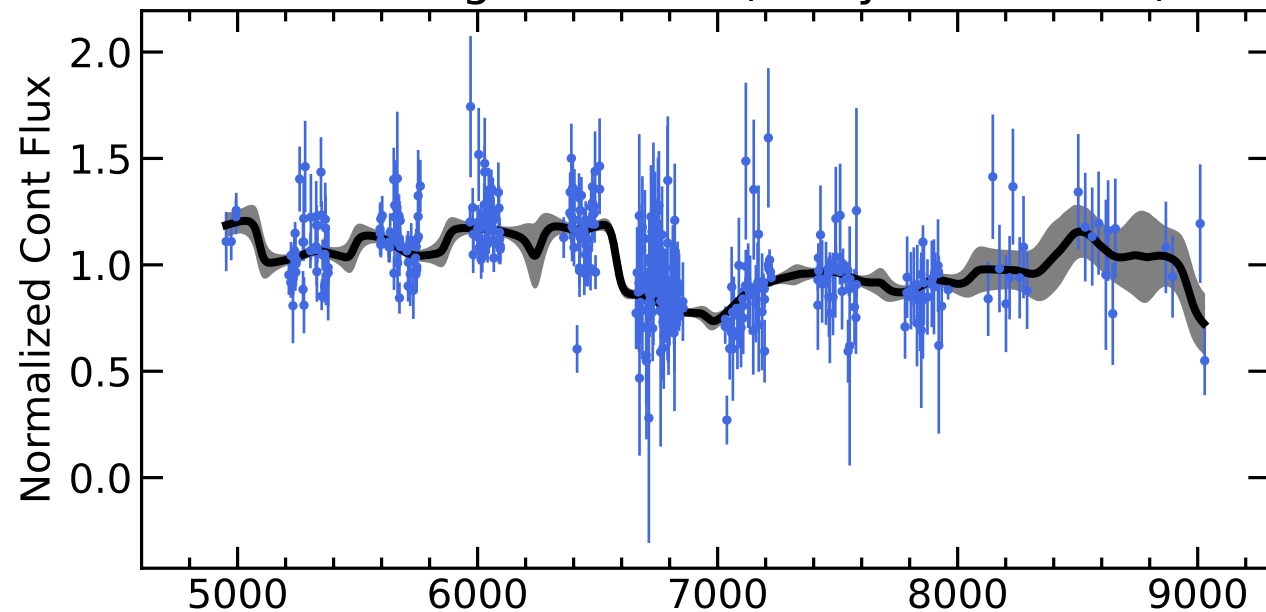
RM002 Light Curves (w/ PyROA model)
