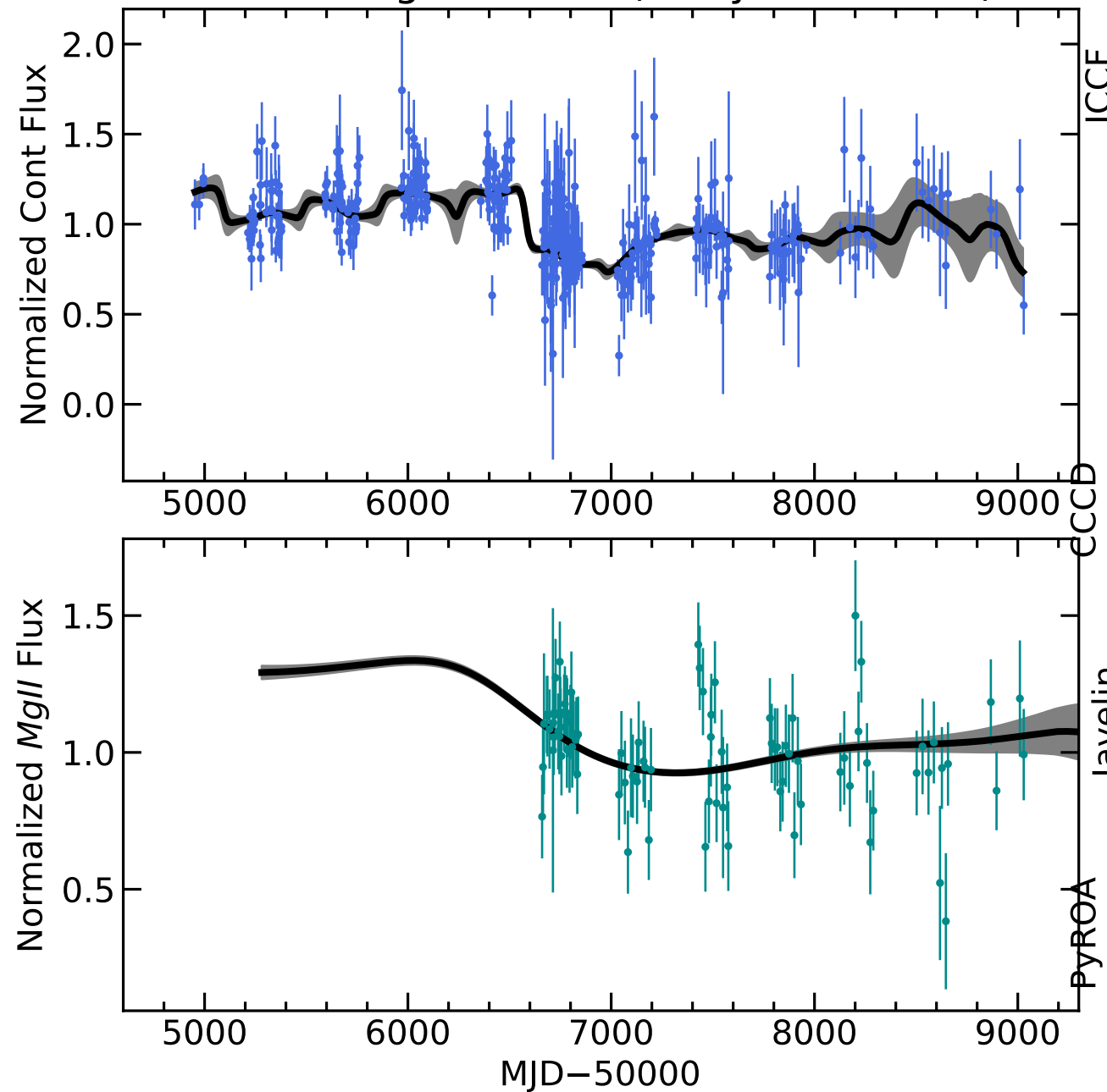
RM002 Light Curves (w/ PyROA model)
