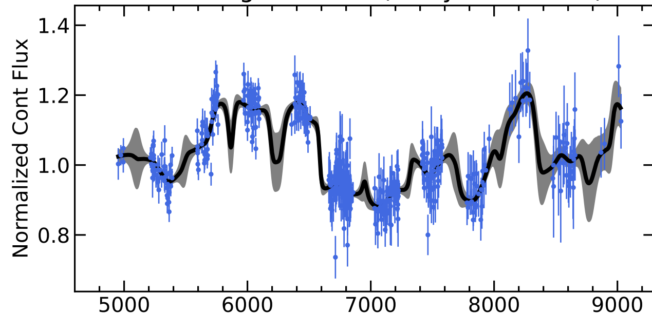
RM003 Light Curves (w/ PyROA model)
