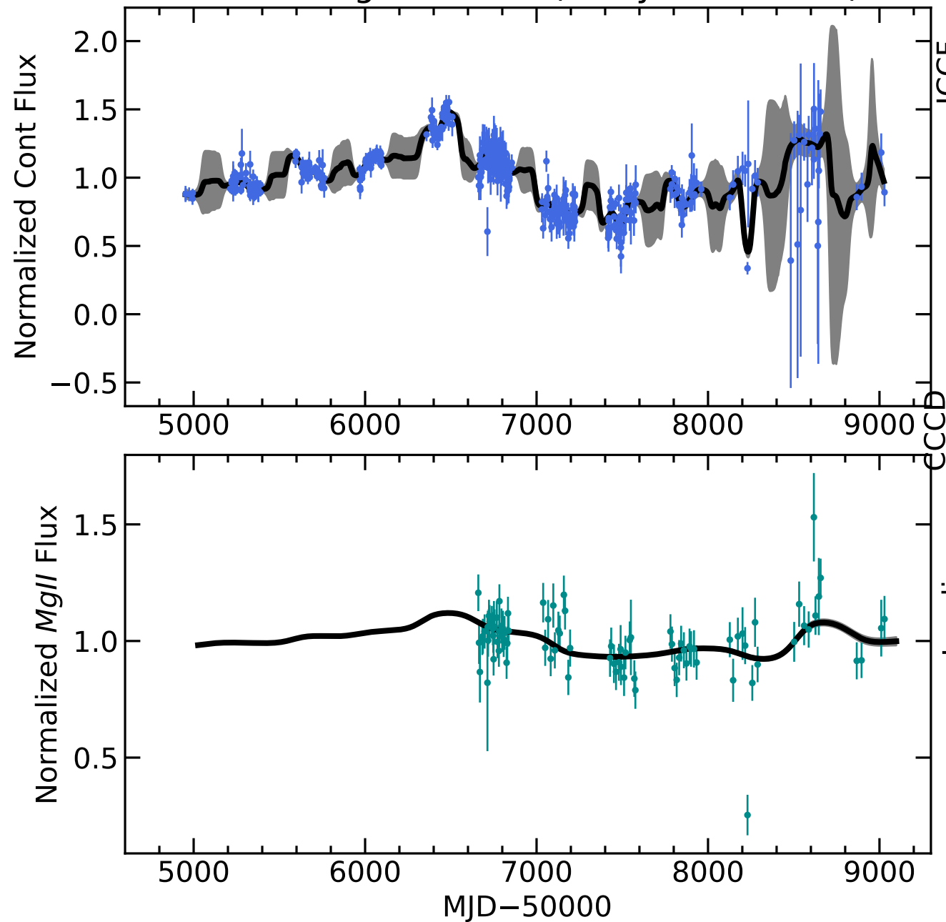
RM006 Light Curves (w/ PyROA model)
