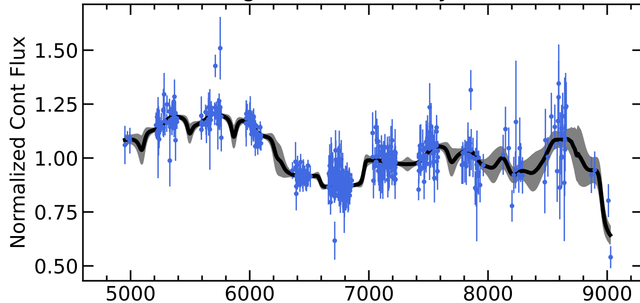
RM008 Light Curves (w/ PyROA model)
