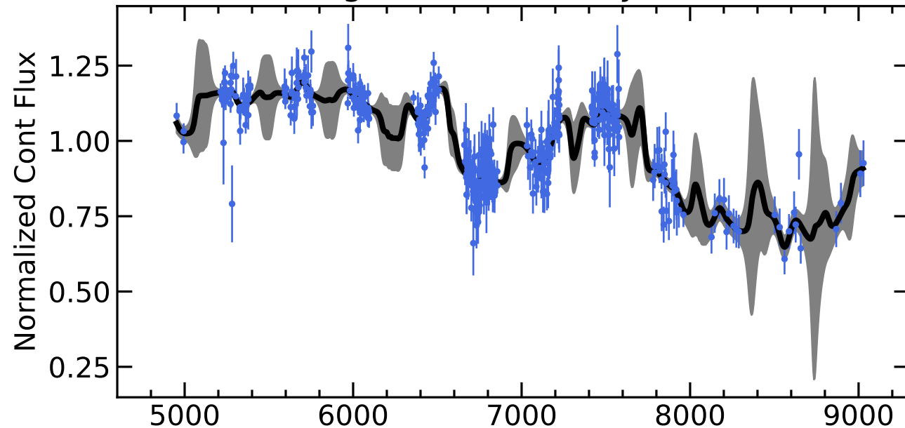
RM009 Light Curves (w/ PyROA model)
