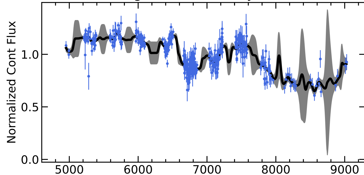
RM009 Light Curves (w/ PyROA model)
