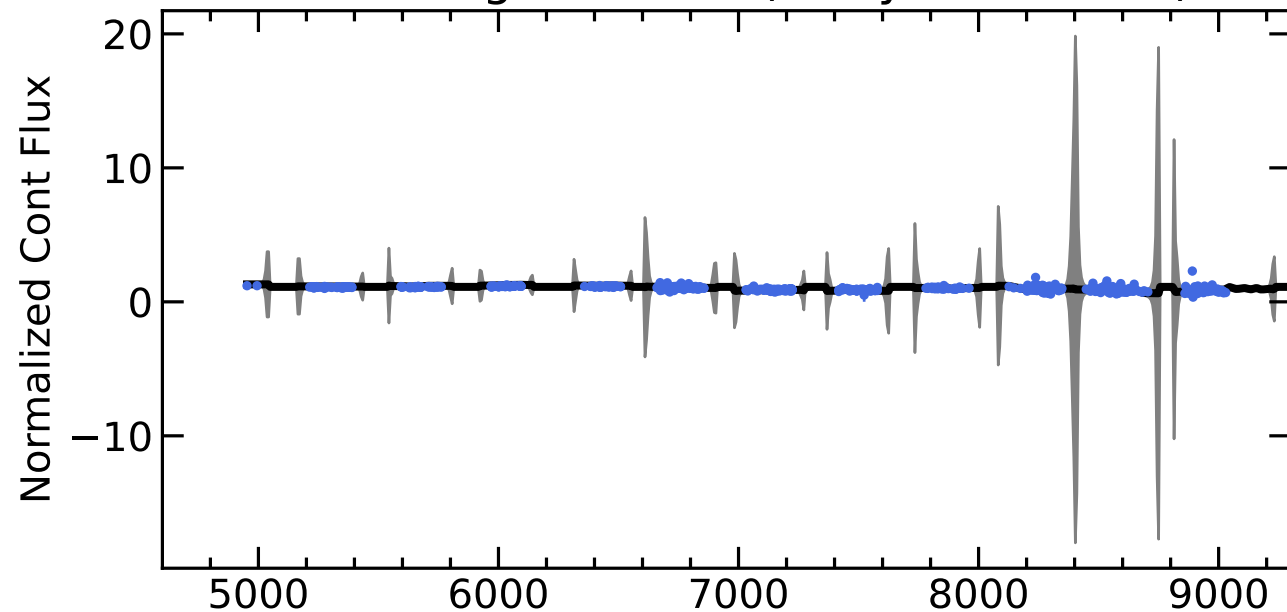
RM010 Light Curves (w/ PyROA model)
