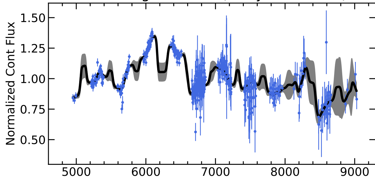
RM011 Light Curves (w/ PyROA model)
