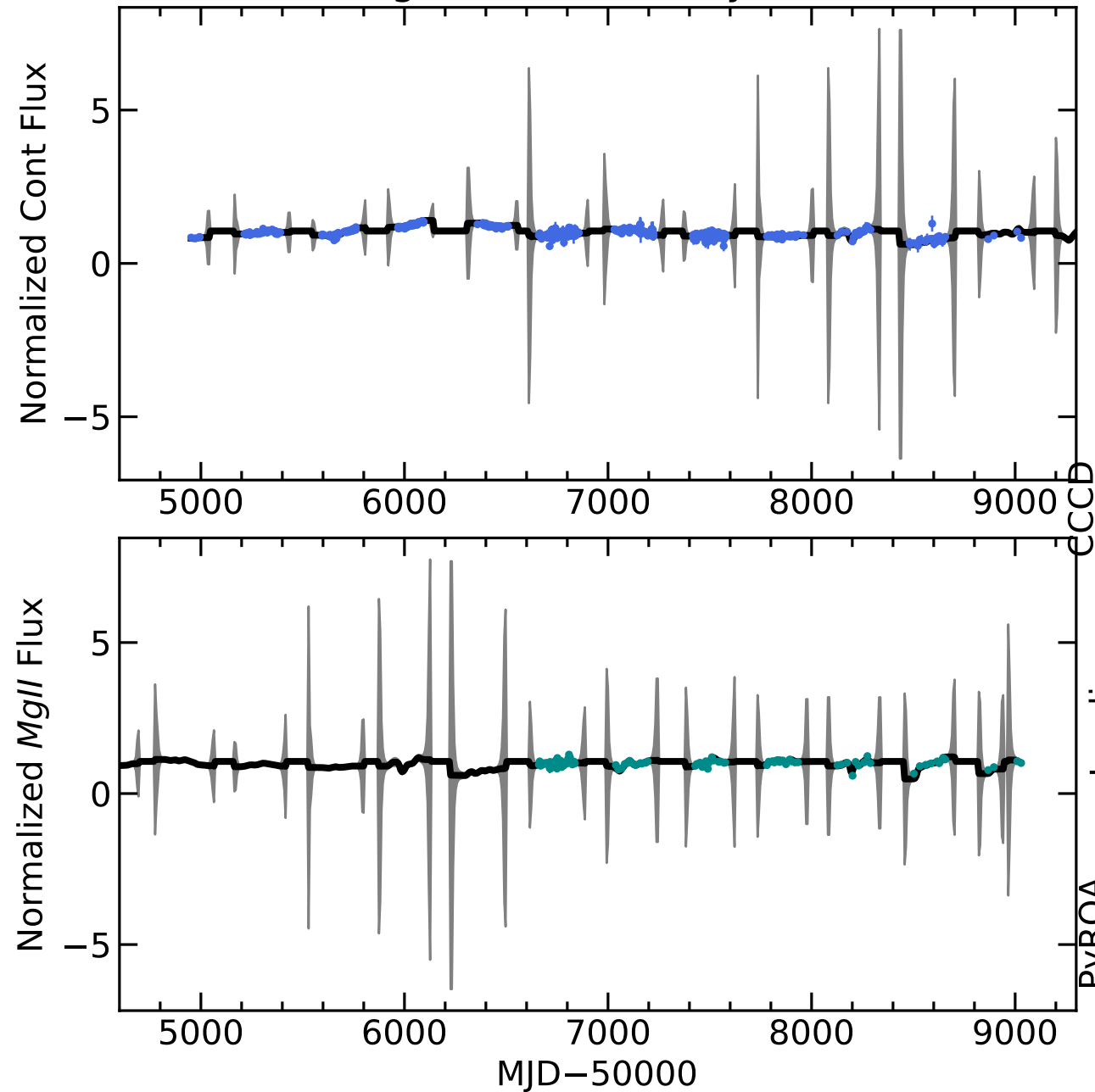
RM011 Light Curves (w/ PyROA model)
