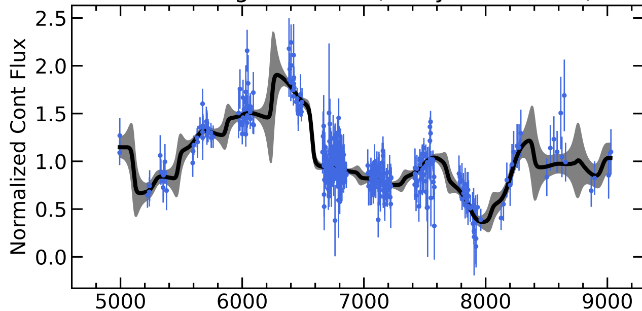
RM012 Light Curves (w/ PyROA model)
