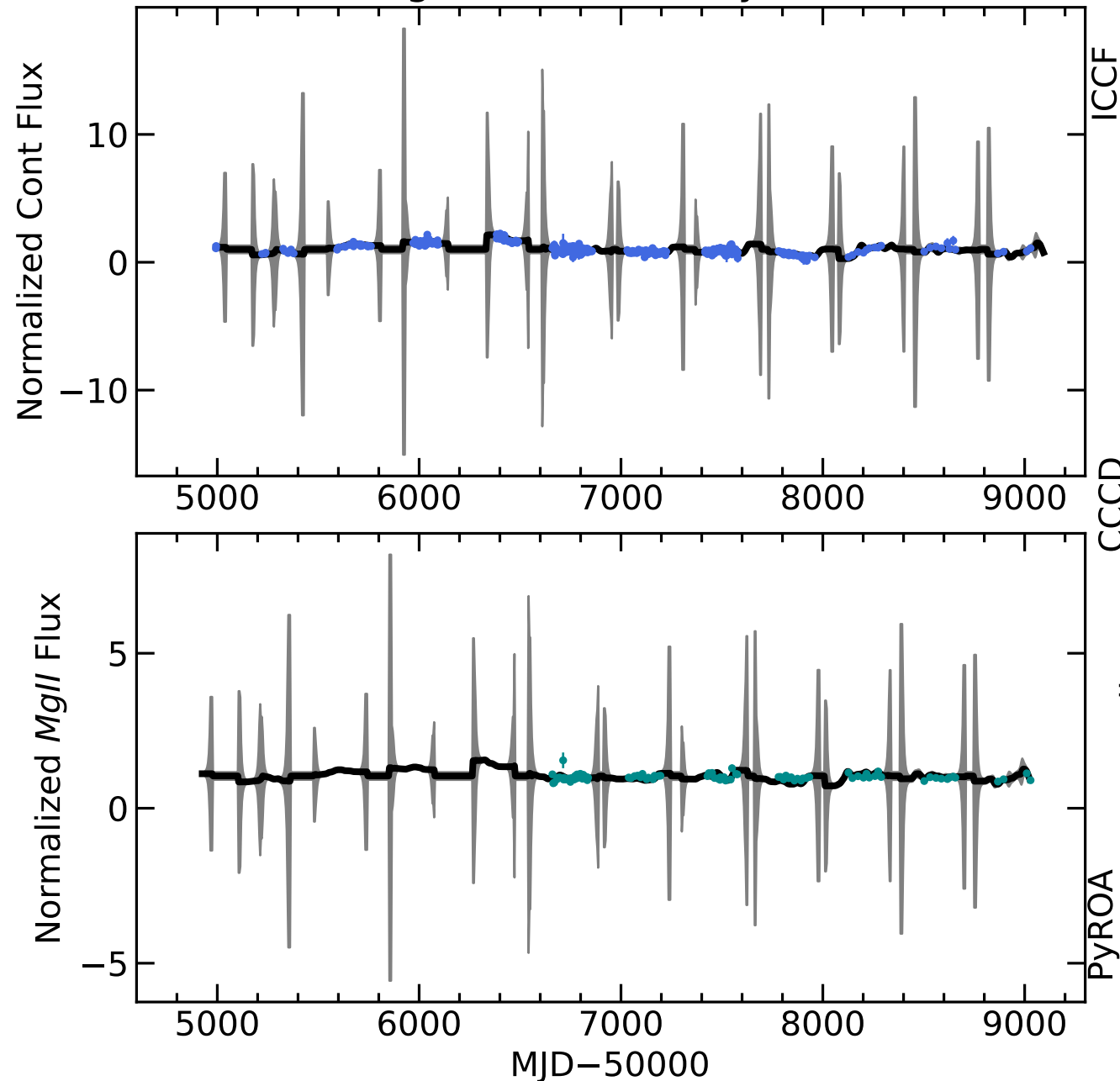
RM012 Light Curves (w/ PyROA model)
