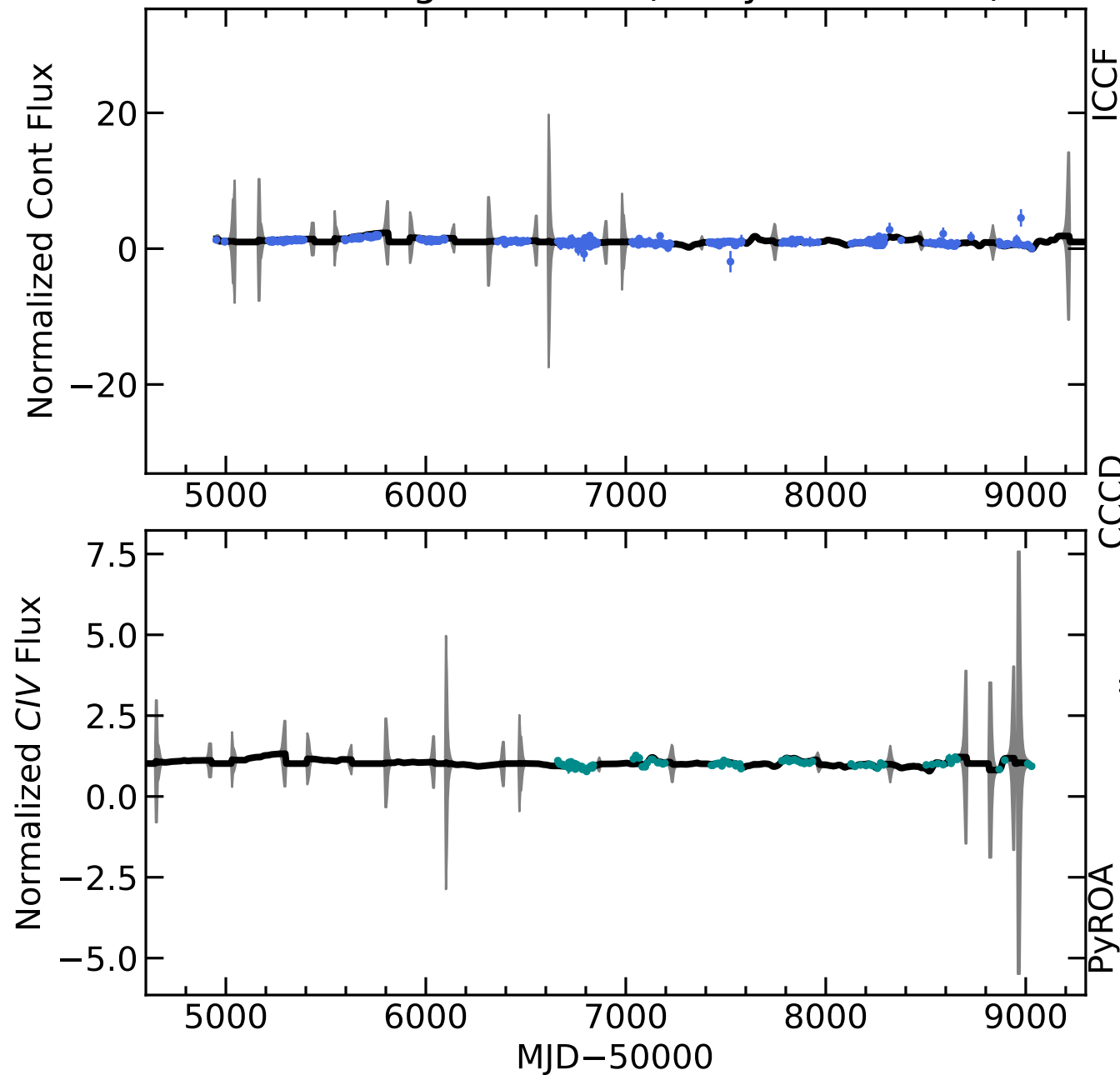
RM013 Light Curves (w/ PyROA model)
