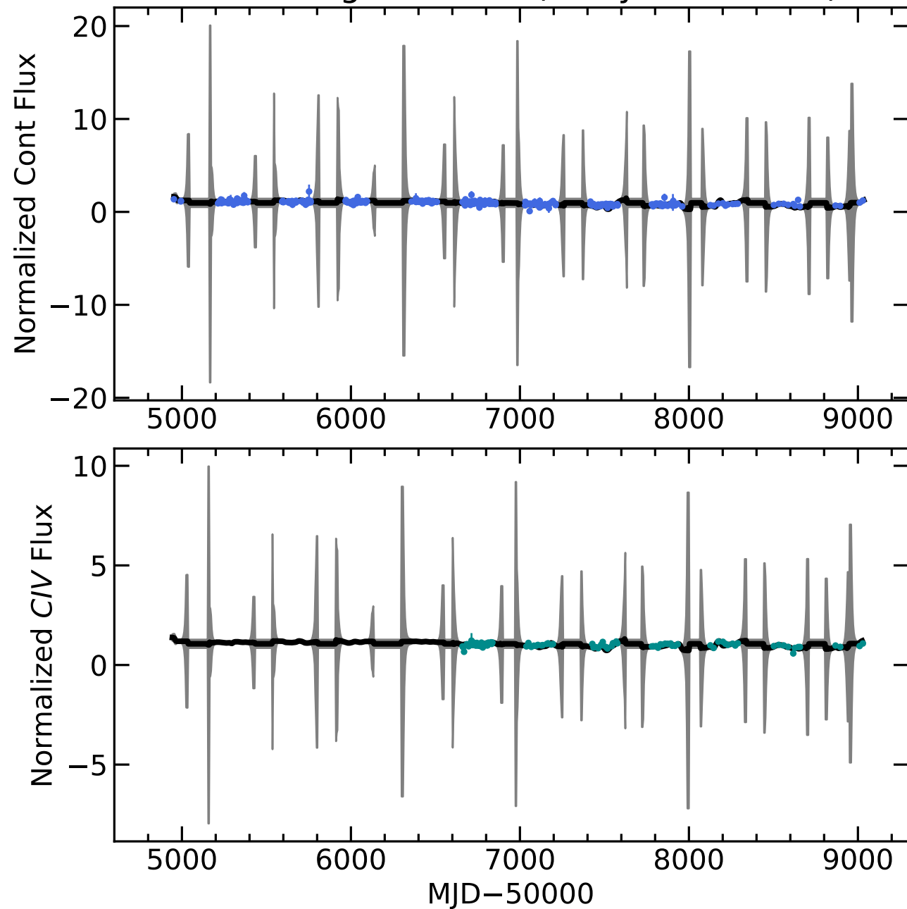
RM014 Light Curves (w/ PyROA model)
