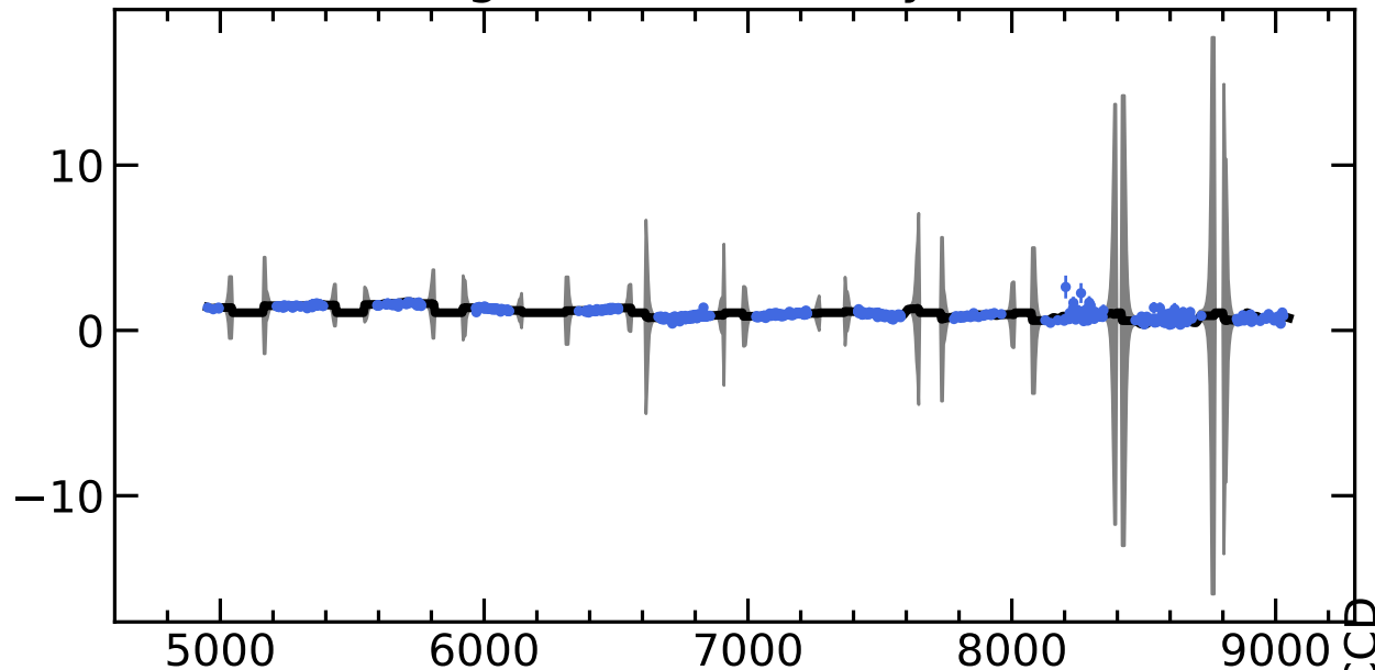
RM015 Light Curves (w/ PyROA model)
