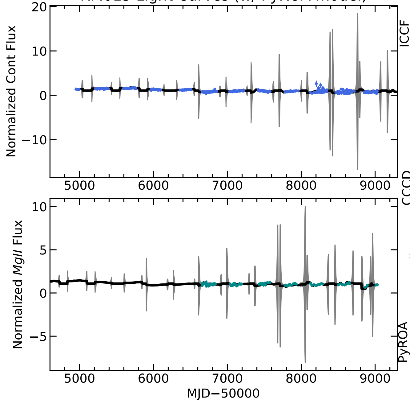
RM015 Light Curves (w/ PyROA model)
