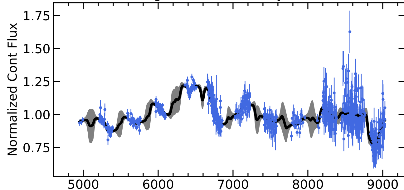
RM016 Light Curves (w/ PyROA model)
