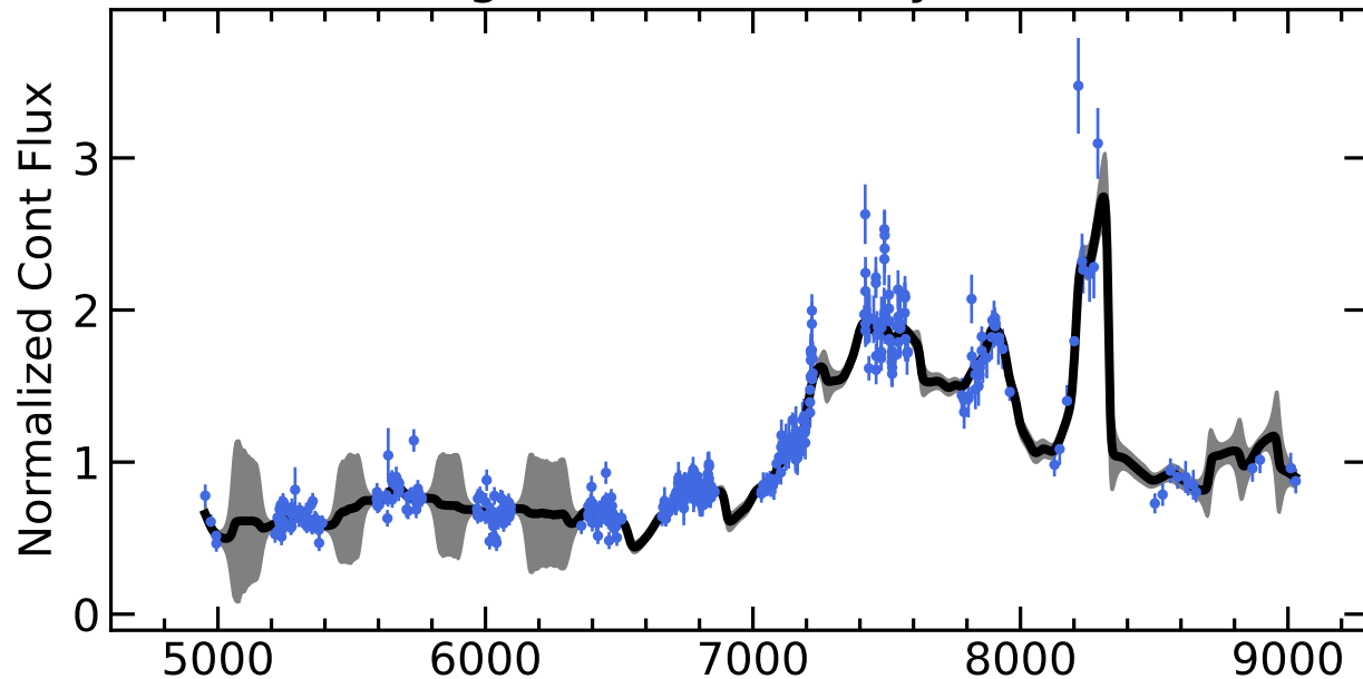
RM017 Light Curves (w/ PyROA model)
