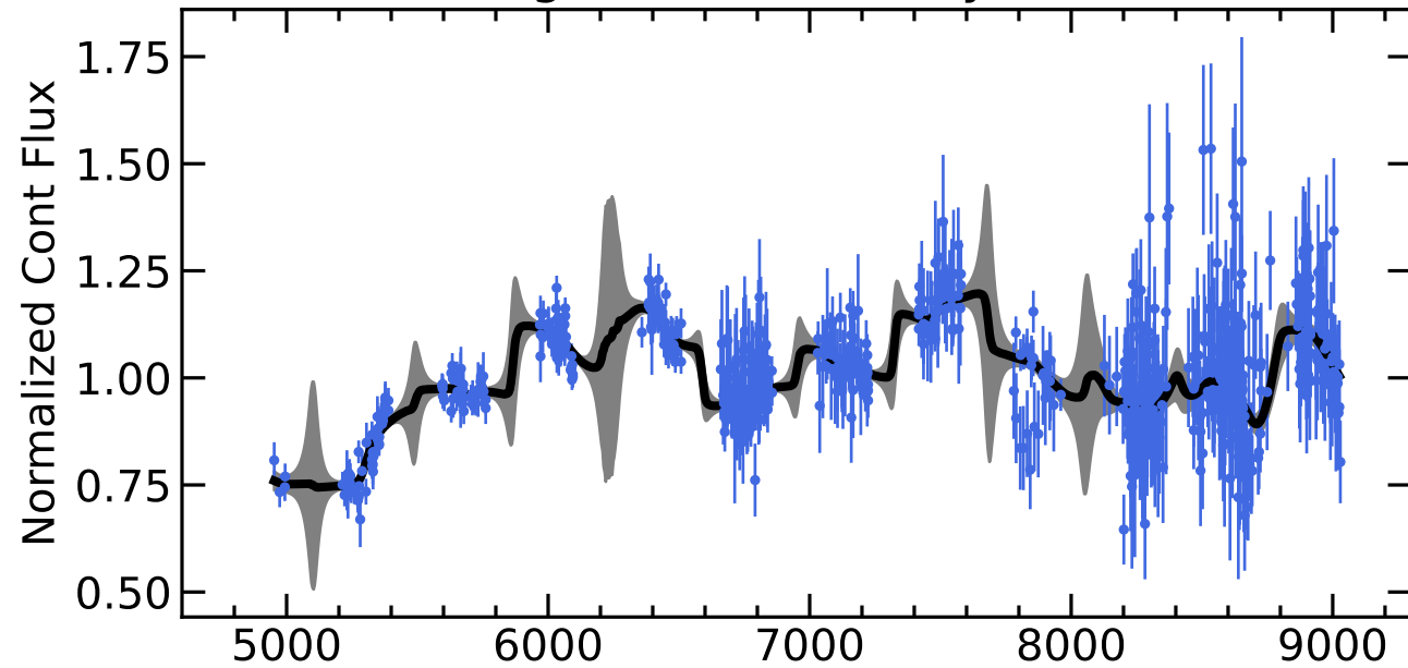
RM019 Light Curves (w/ PyROA model)
