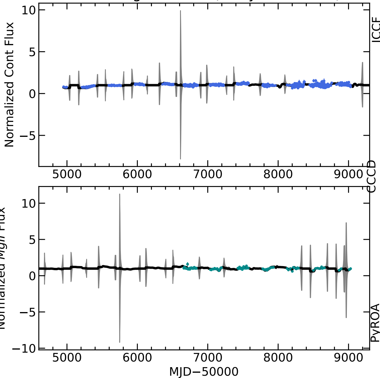
RM019 Light Curves (w/ PyROA model)
