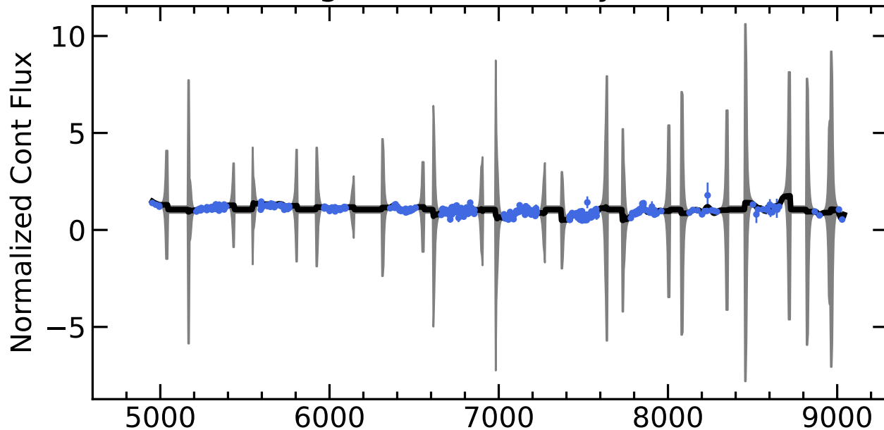
RM021 Light Curves (w/ PyROA model)
