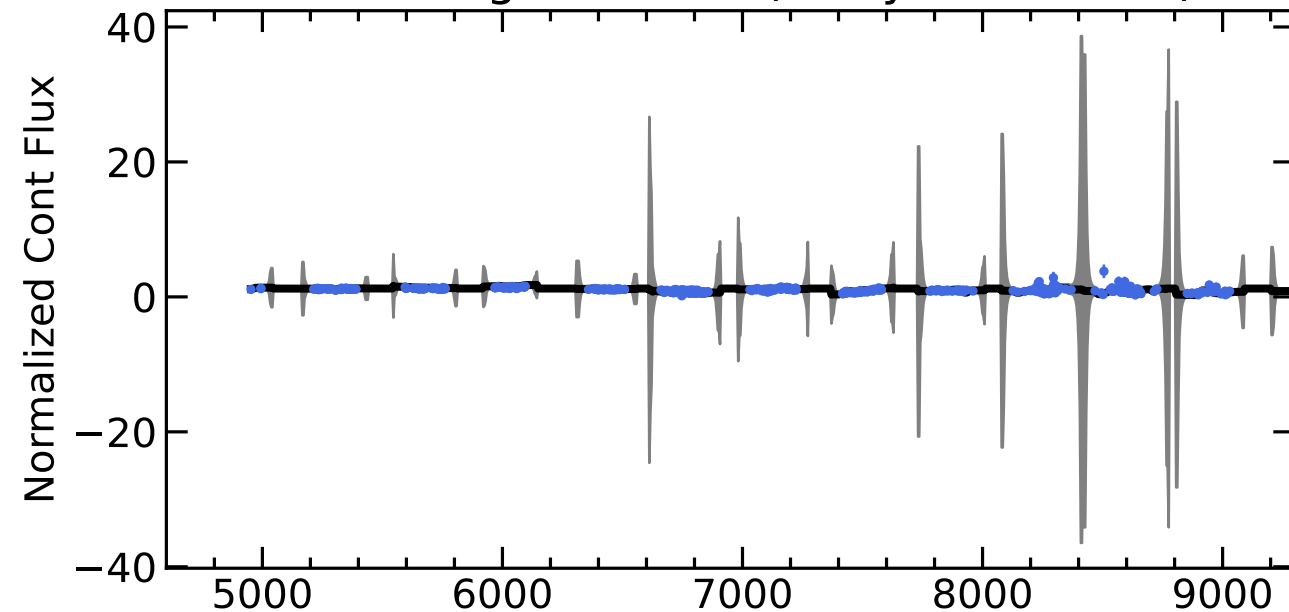
RM022 Light Curves (w/ PyROA model)
