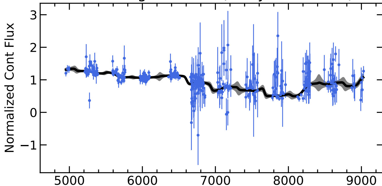
RM023 Light Curves (w/ PyROA model)
