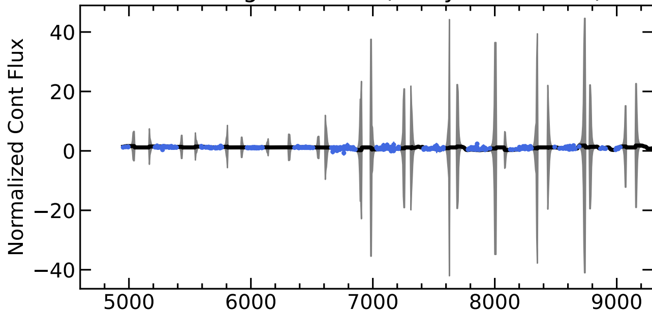
RM023 Light Curves (w/ PyROA model)
