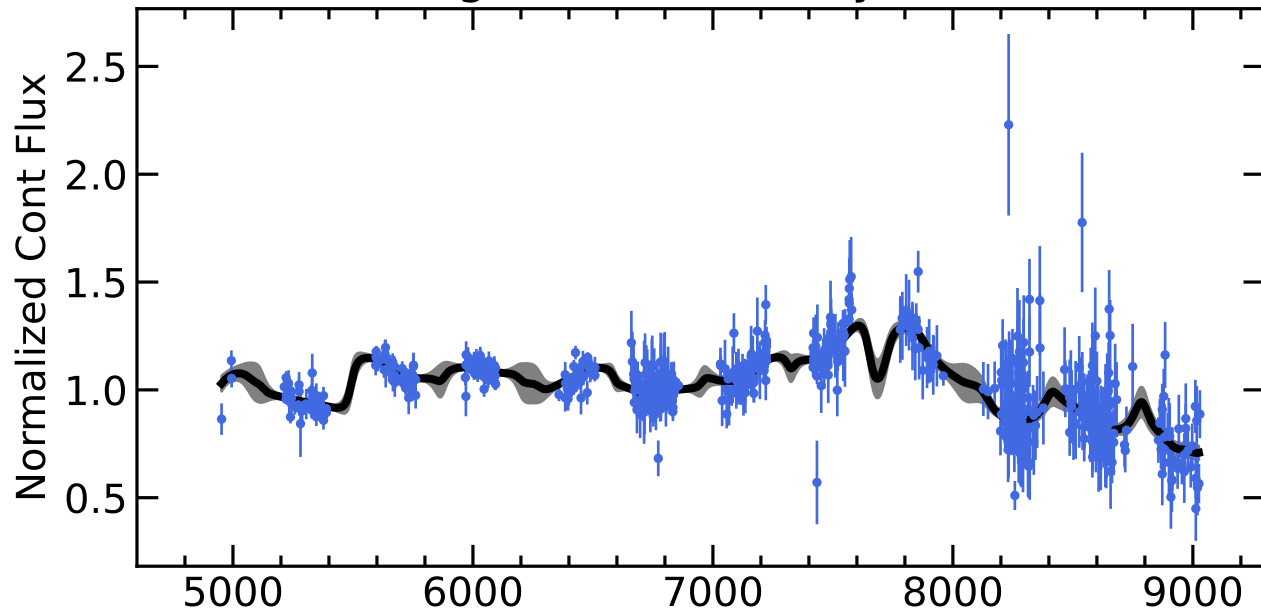
RM025 Light Curves (w/ PyROA model)
