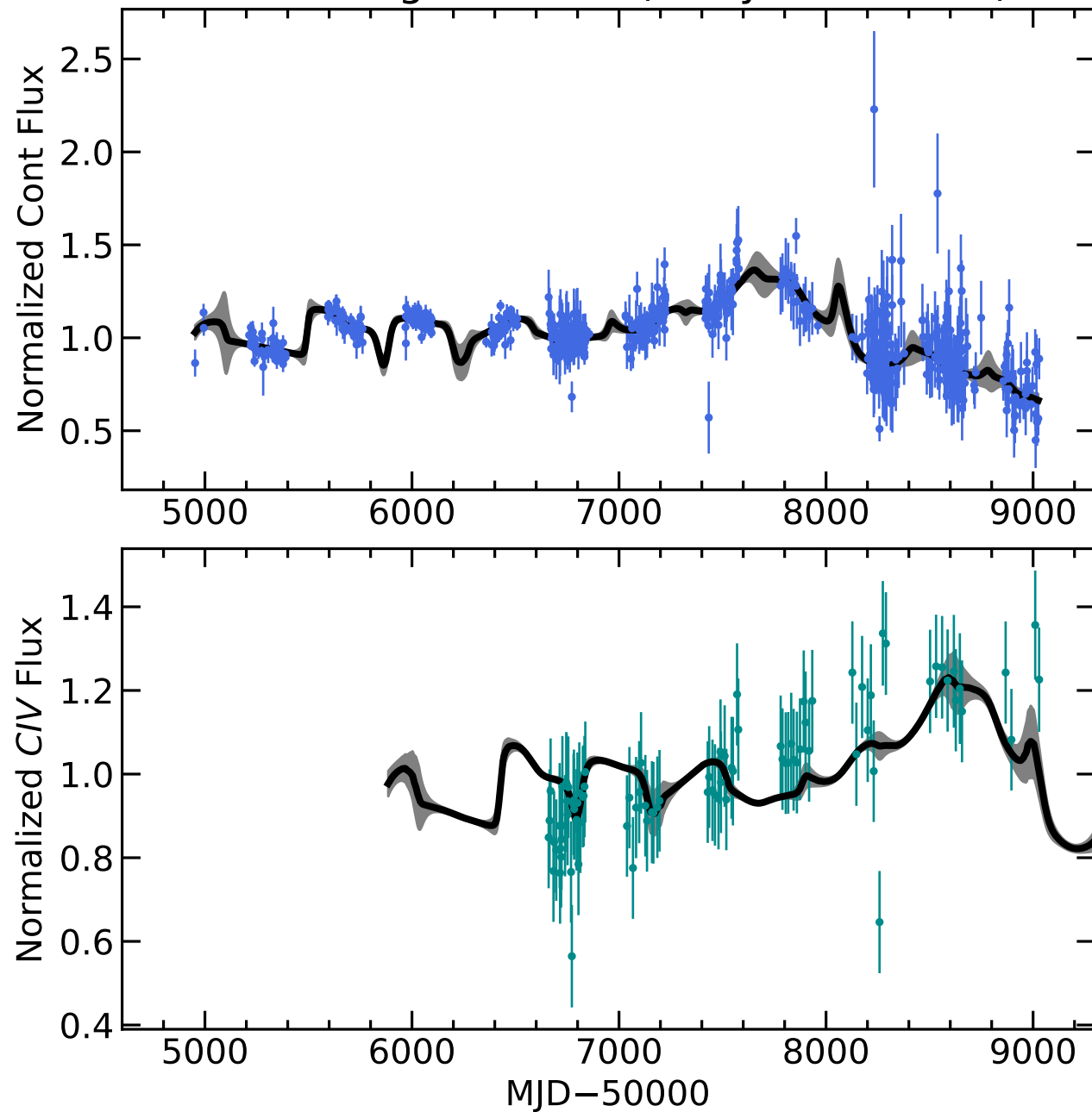
RM025 Light Curves (w/ PyROA model)
