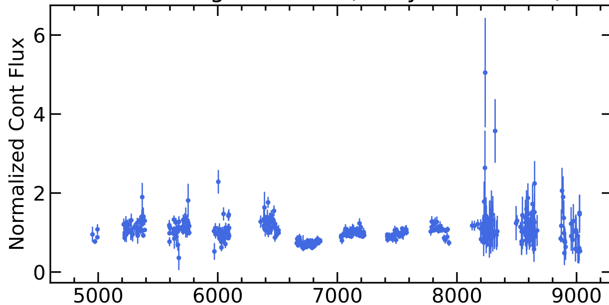
RM027 Light Curves (w/ PyROA model)
