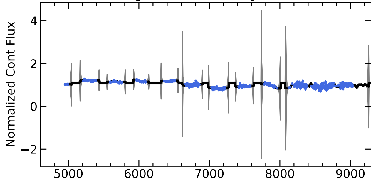
RM028 Light Curves (w/ PyROA model)
