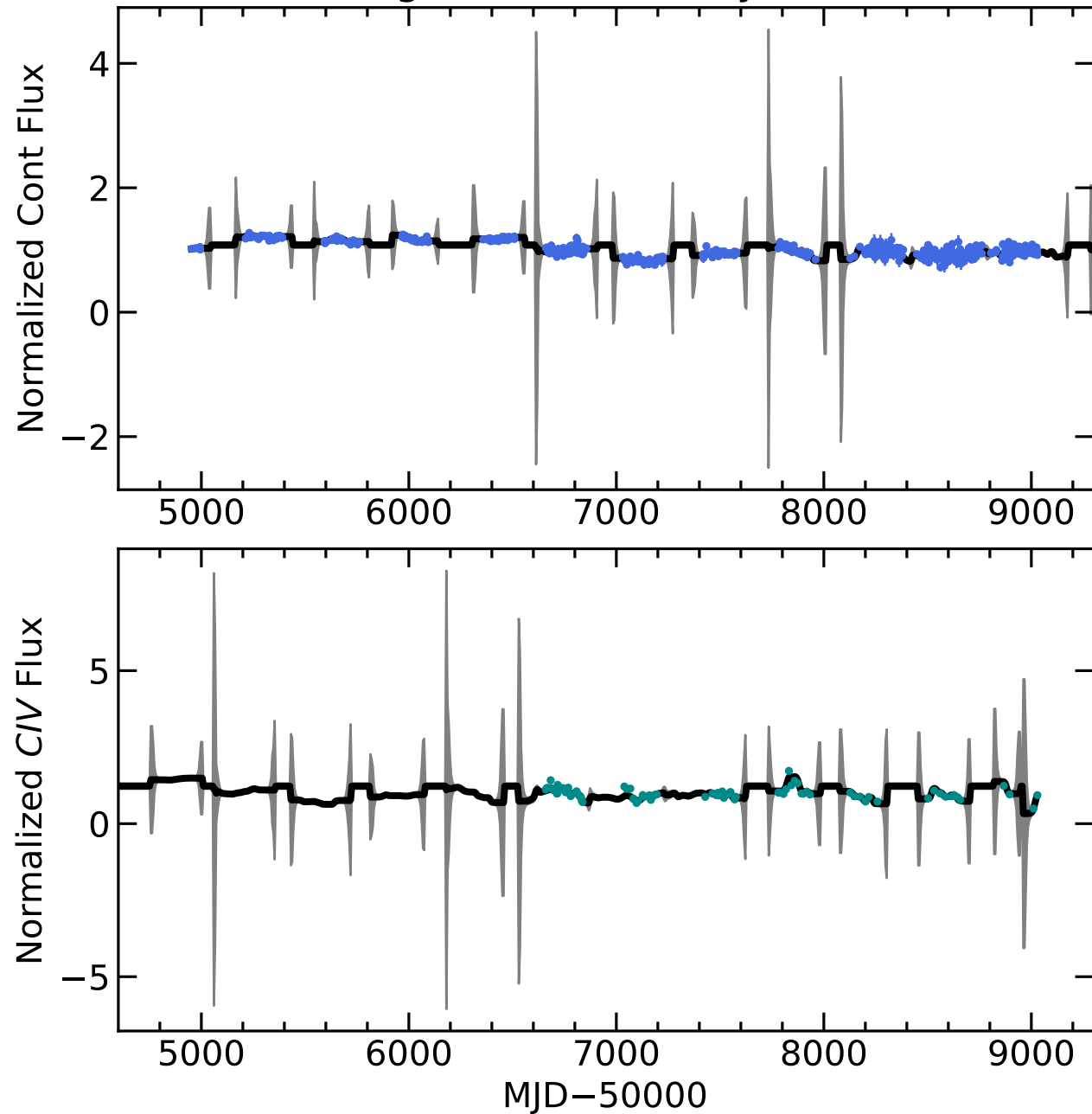
RM028 Light Curves (w/ PyROA model)
