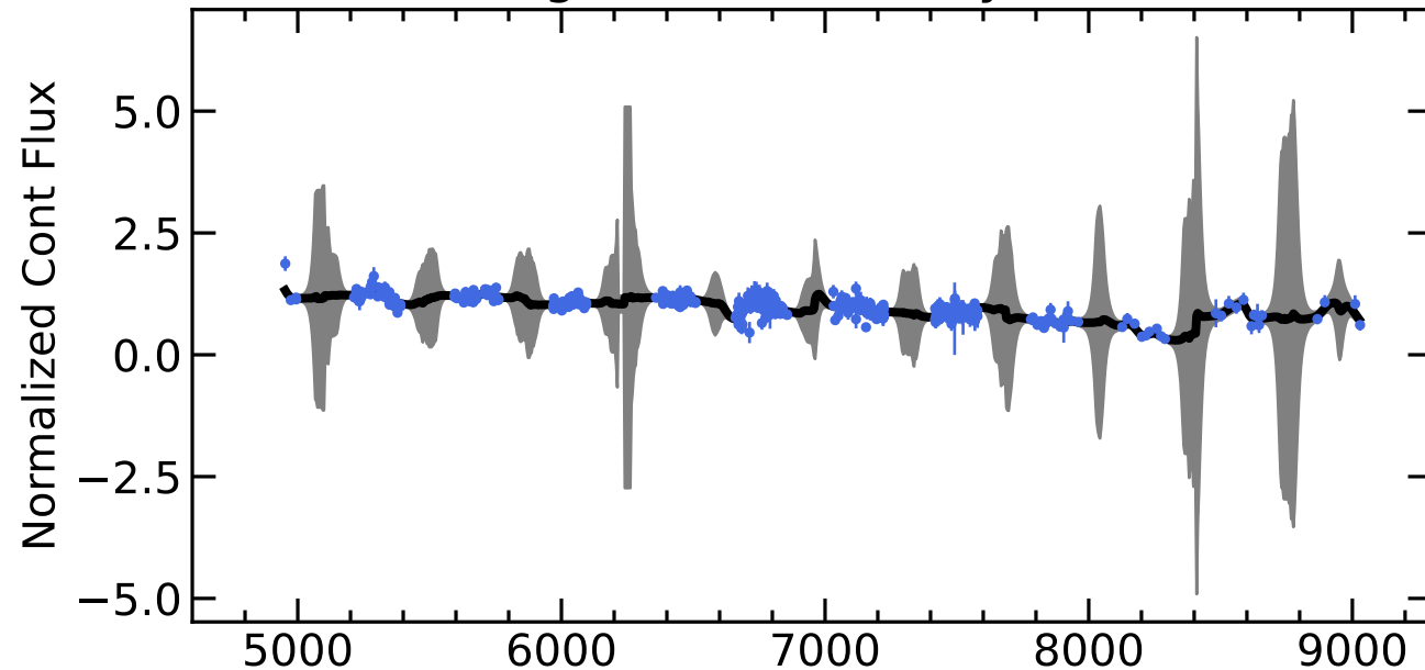
RM029 Light Curves (w/ PyROA model)
