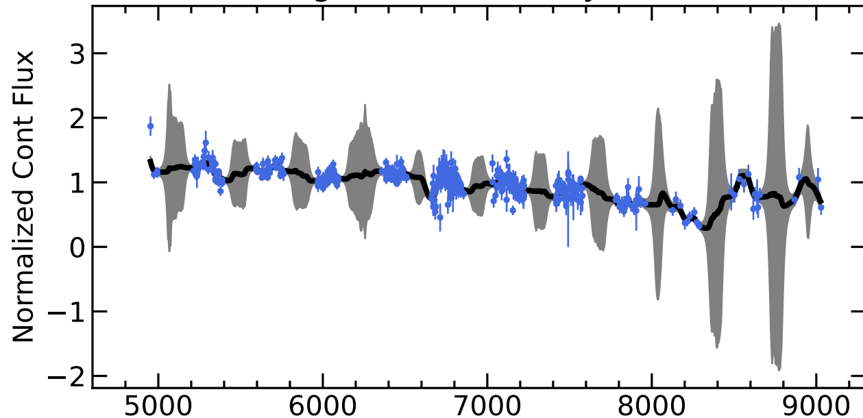
RM029 Light Curves (w/ PyROA model)
