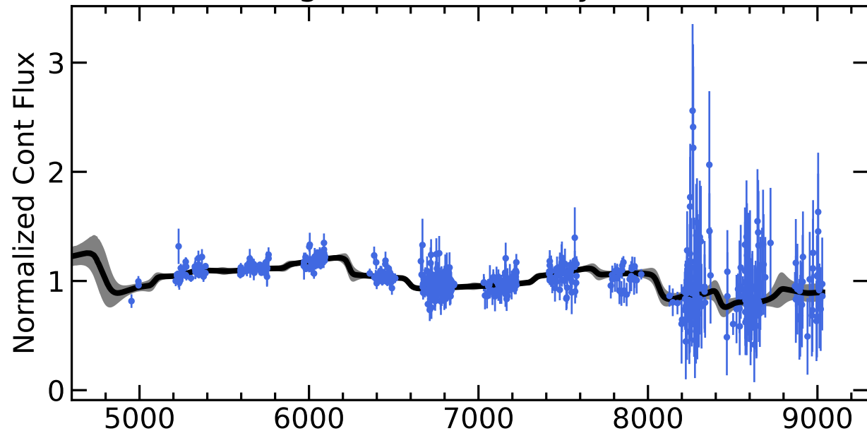
RM030 Light Curves (w/ PyROA model)
