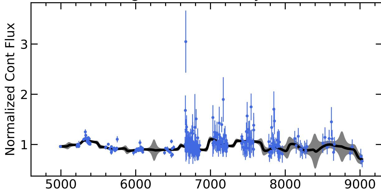
RM033 Light Curves (w/ PyROA model)
