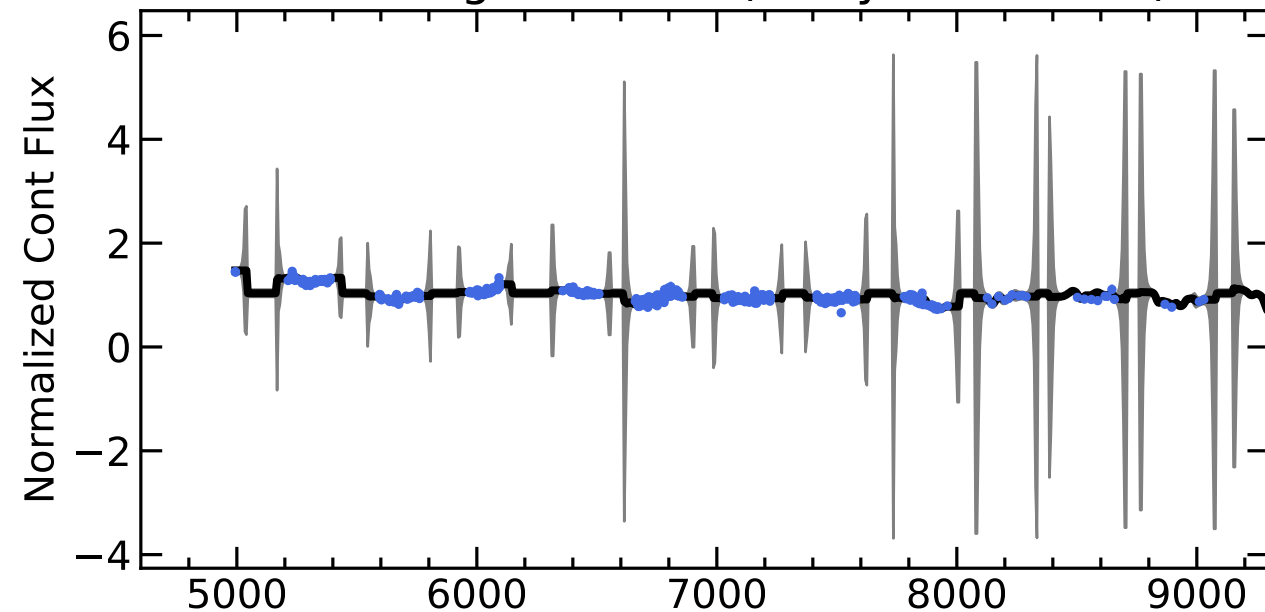
RM034 Light Curves (w/ PyROA model)
