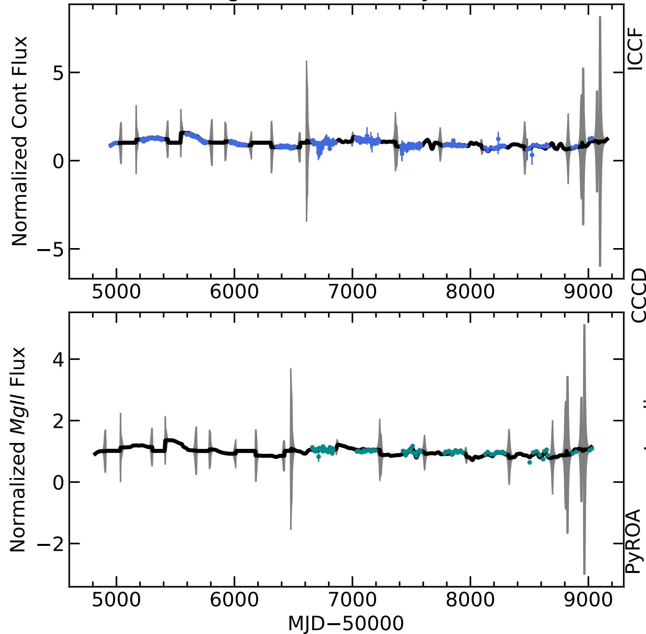
RM037 Light Curves (w/ PyROA model)
