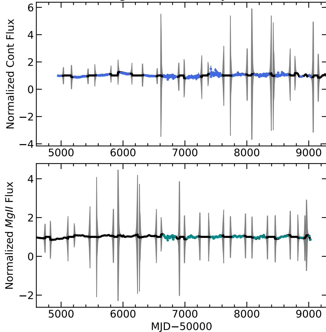
RM038 Light Curves (w/ PyROA model)
