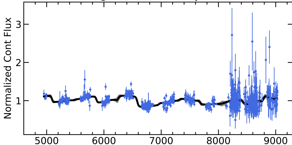
RM039 Light Curves (w/ PyROA model)
