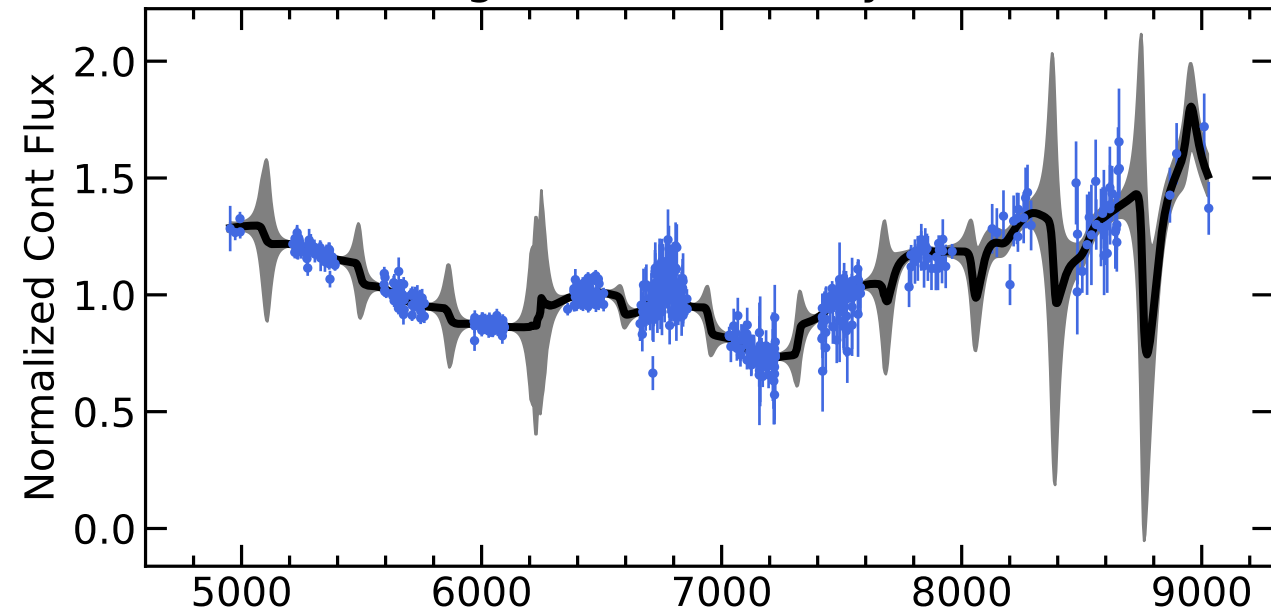
RM041 Light Curves (w/ PyROA model)
