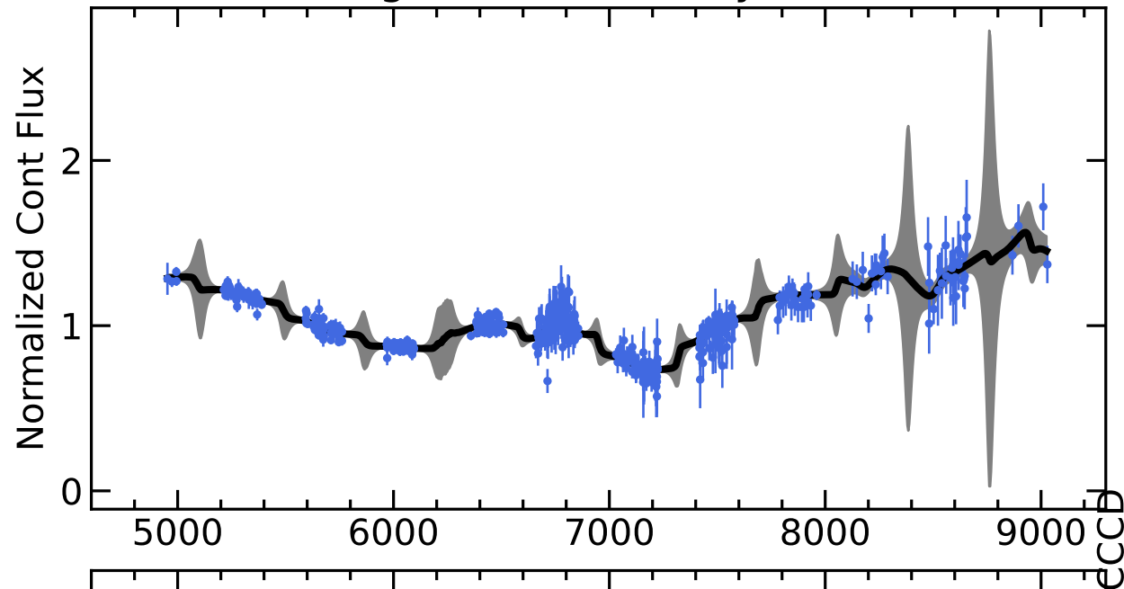
RM041 Light Curves (w/ PyROA model)
