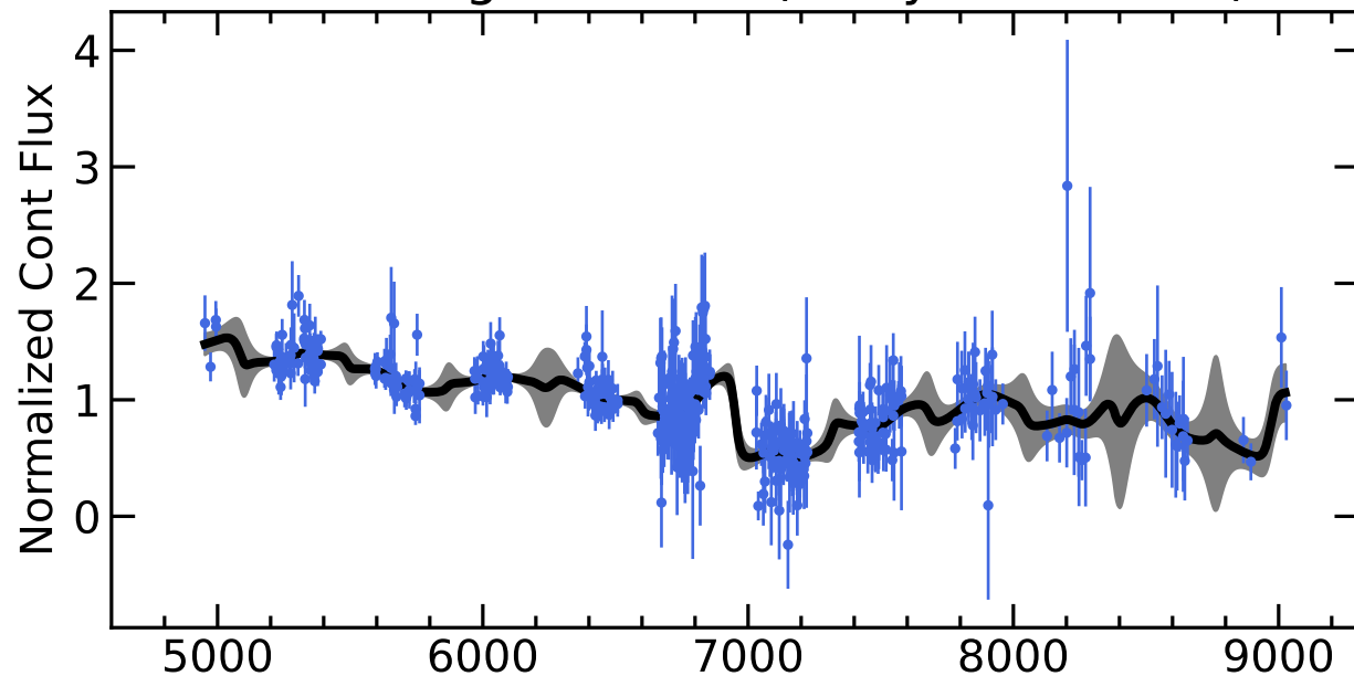
RM042 Light Curves (w/ PyROA model)
