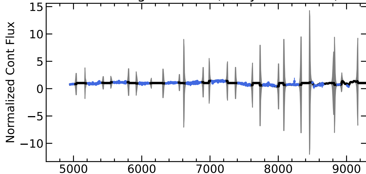
RM043 Light Curves (w/ PyROA model)
