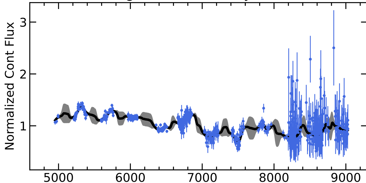
RM044 Light Curves (w/ PyROA model)
