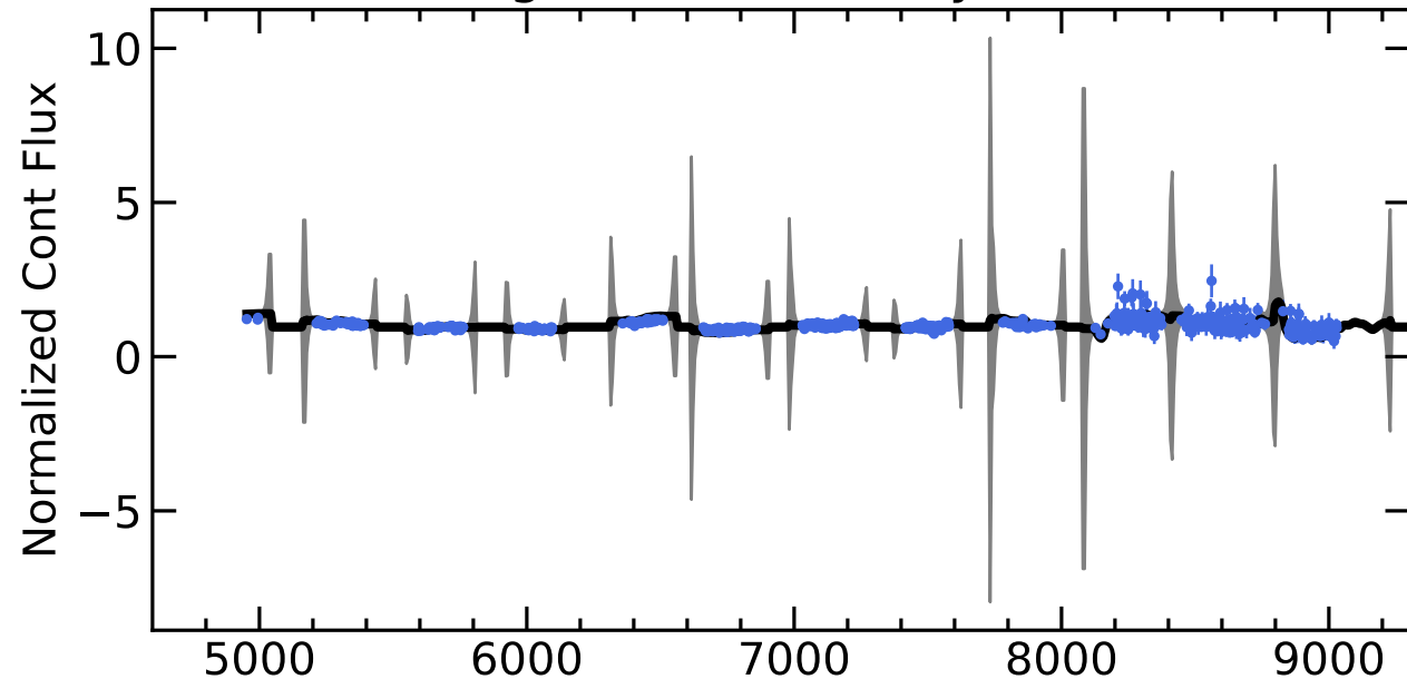
RM048 Light Curves (w/ PyROA model)
