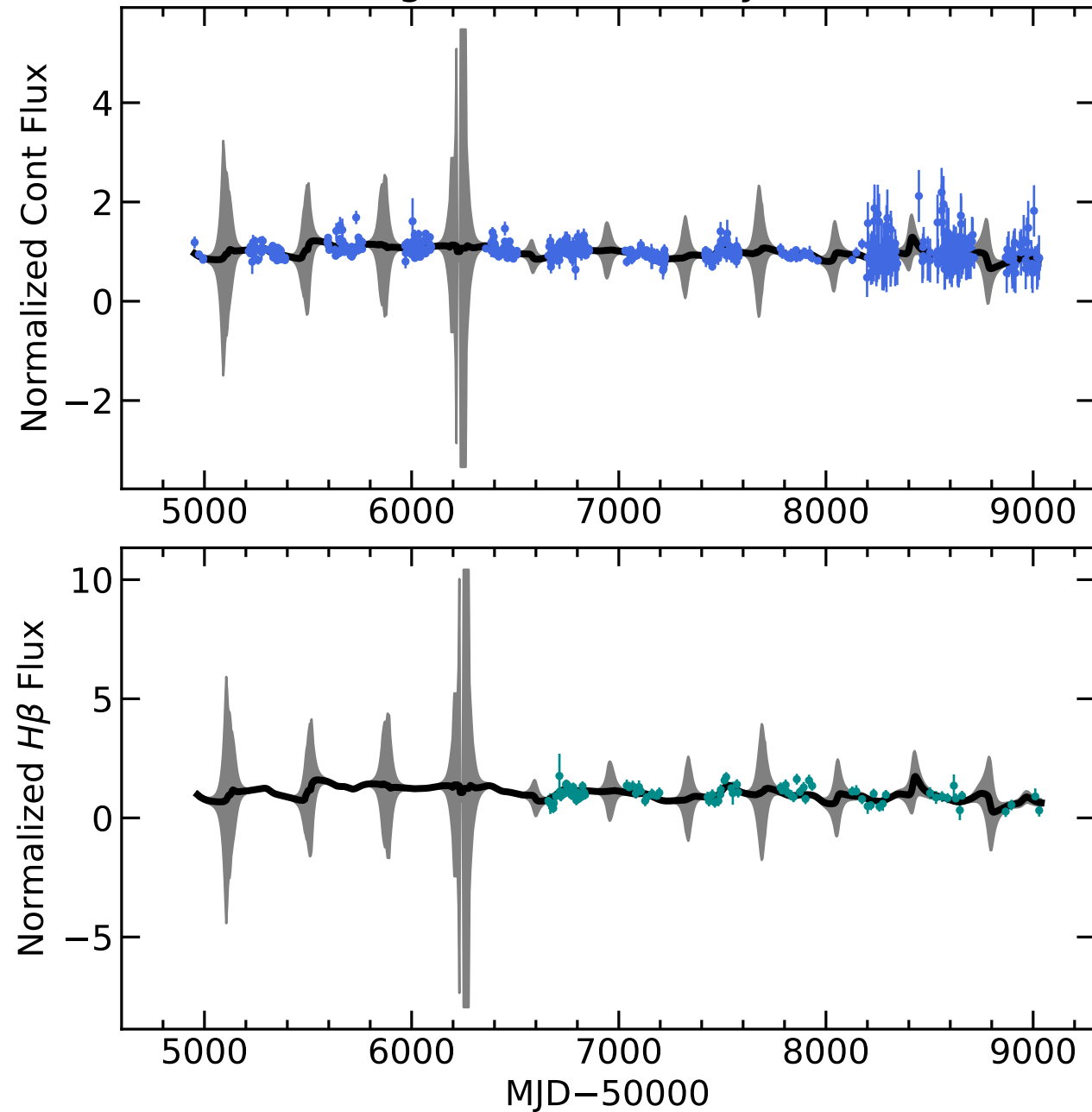
RM050 Light Curves (w/ PyROA model)
