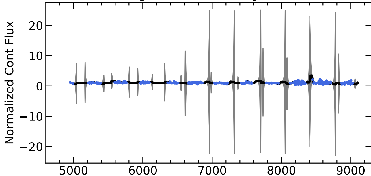
RM050 Light Curves (w/ PyROA model)
