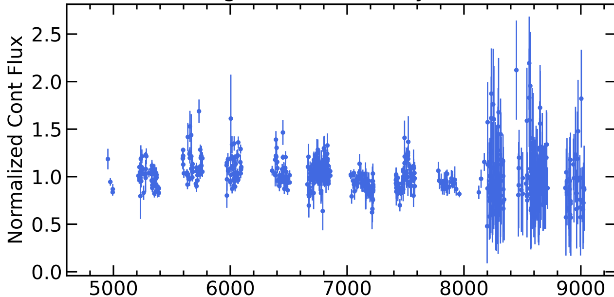
RM050 Light Curves (w/ PyROA model)
