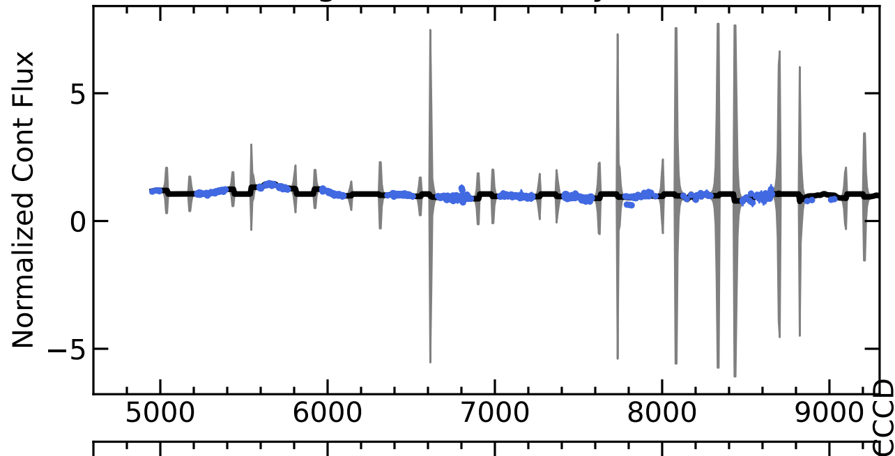
RM051 Light Curves (w/ PyROA model)
