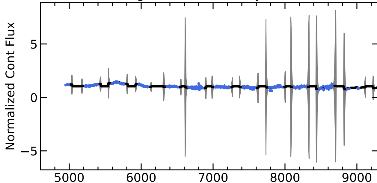
RM051 Light Curves (w/ PyROA model)
