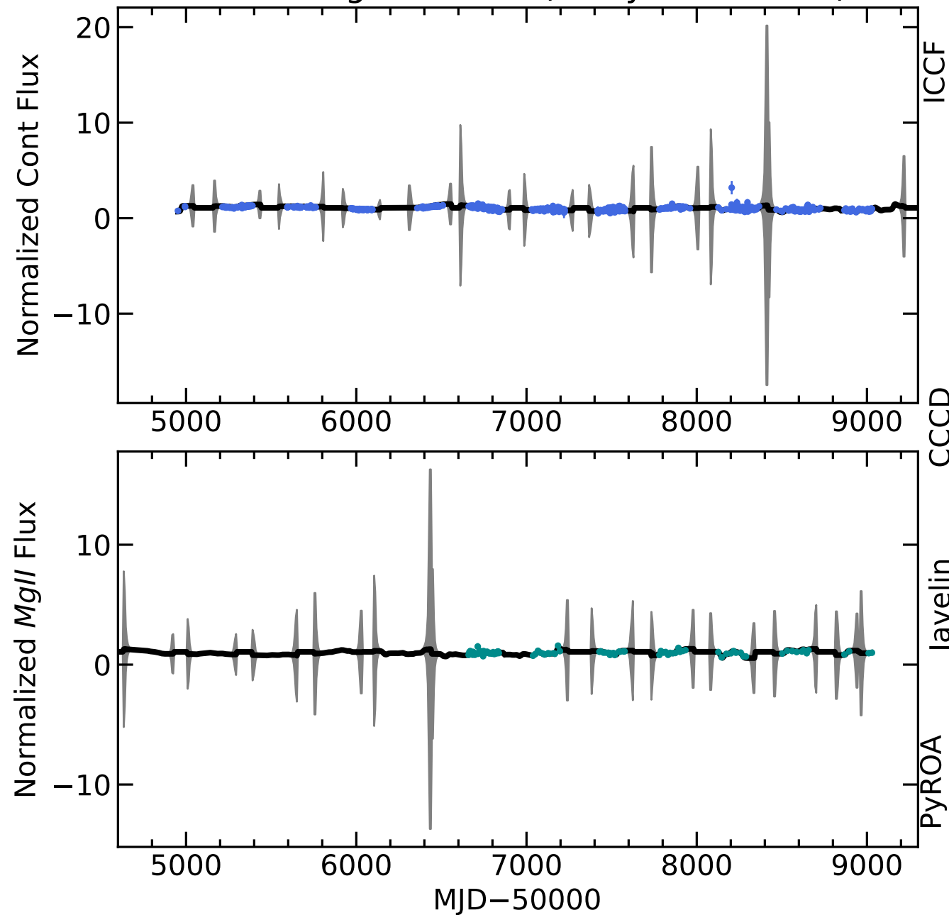
RM052 Light Curves (w/ PyROA model)
