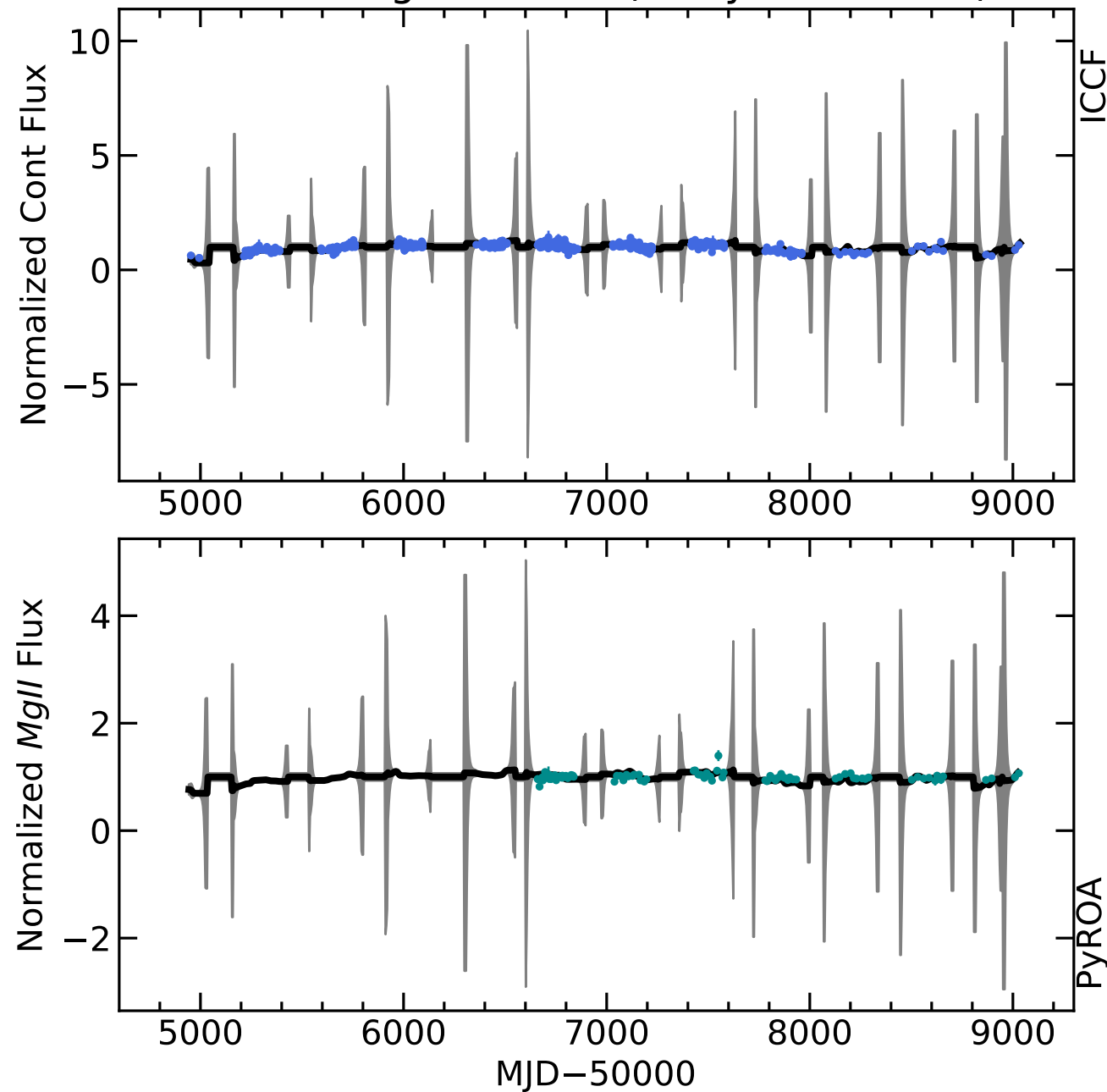
RM053 Light Curves (w/ PyROA model)
