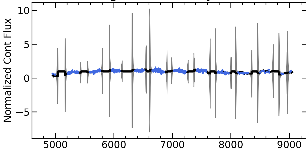
RM053 Light Curves (w/ PyROA model)
