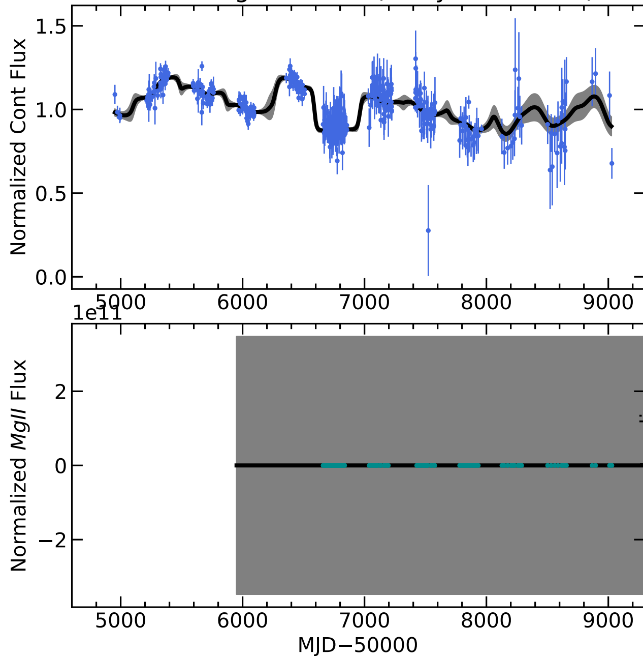
RM054 Light Curves (w/ PyROA model)
