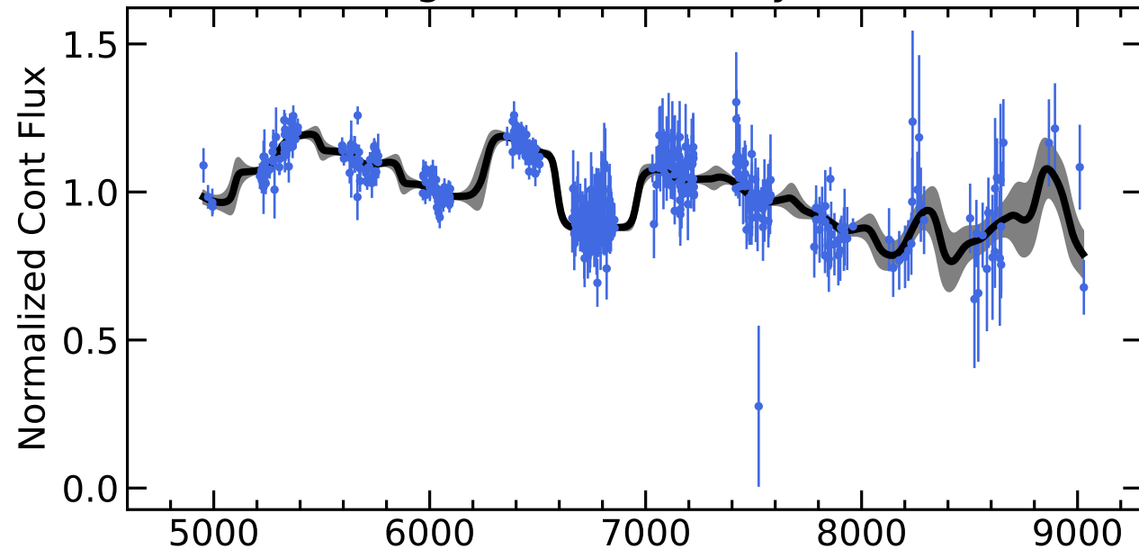
RM054 Light Curves (w/ PyROA model)
