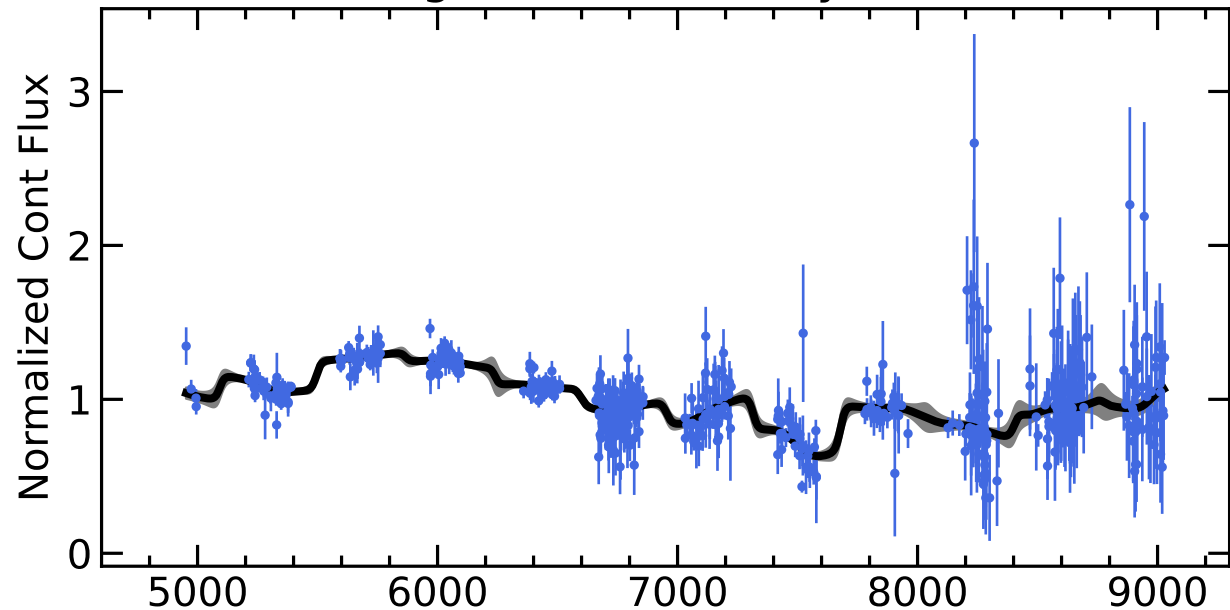
RM056 Light Curves (w/ PyROA model)
