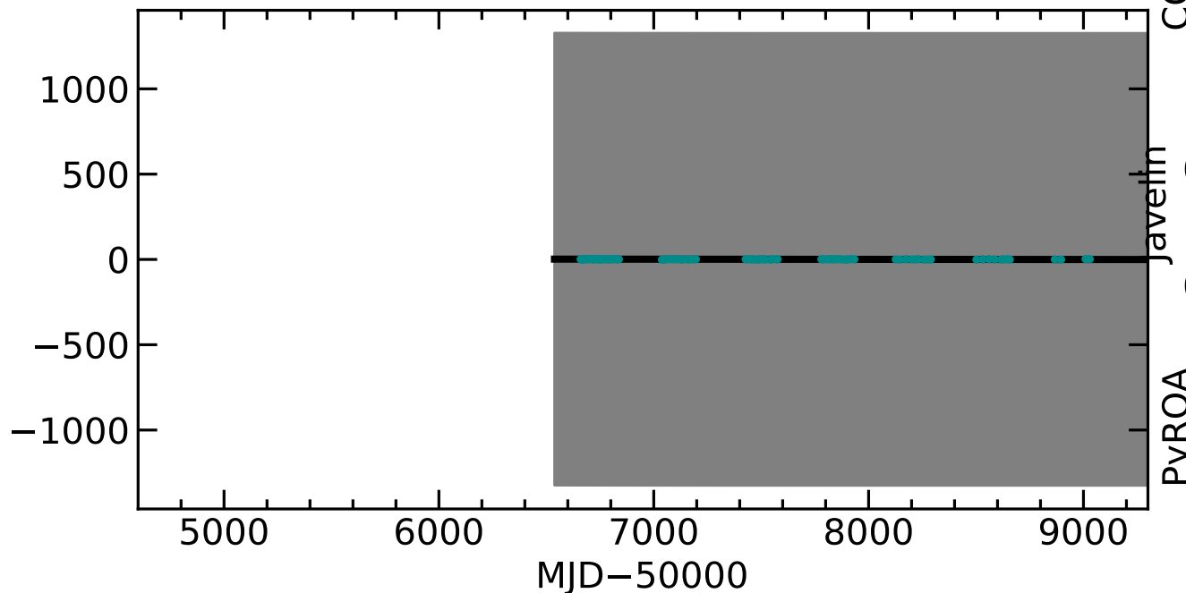
Normalized MgII Flux
