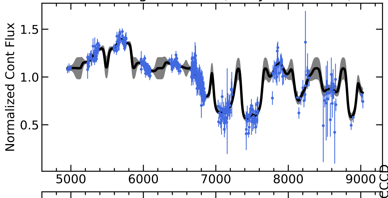
RM057 Light Curves (w/ PyROA model)
