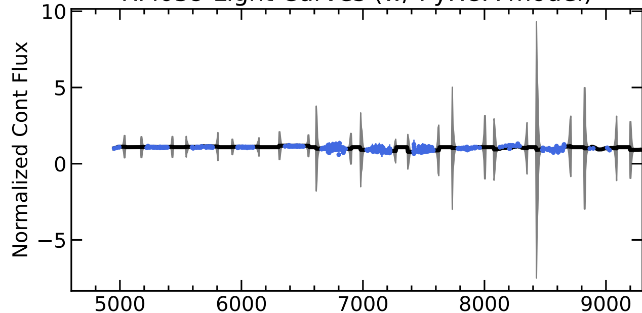
RM059 Light Curves (w/ PyROA model)
