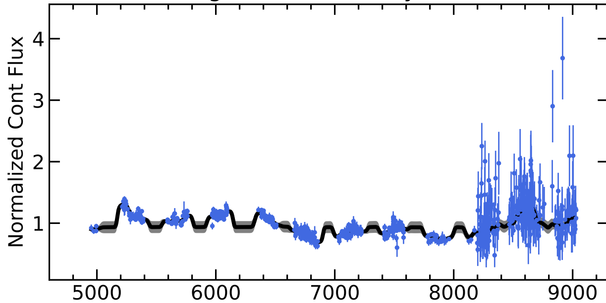
RM062 Light Curves (w/ PyROA model)
