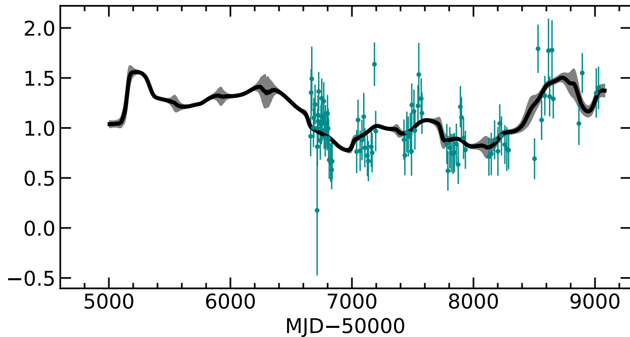
Normalized H\beta Flux
