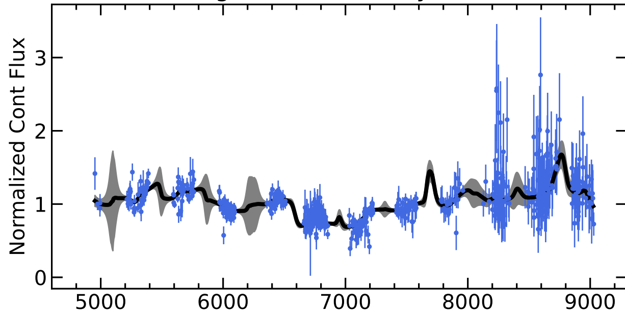
RM063 Light Curves (w/ PyROA model)
