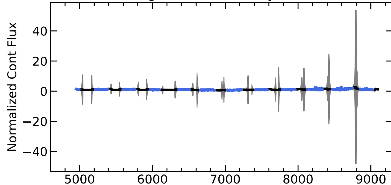
RM063 Light Curves (w/ PyROA model)
