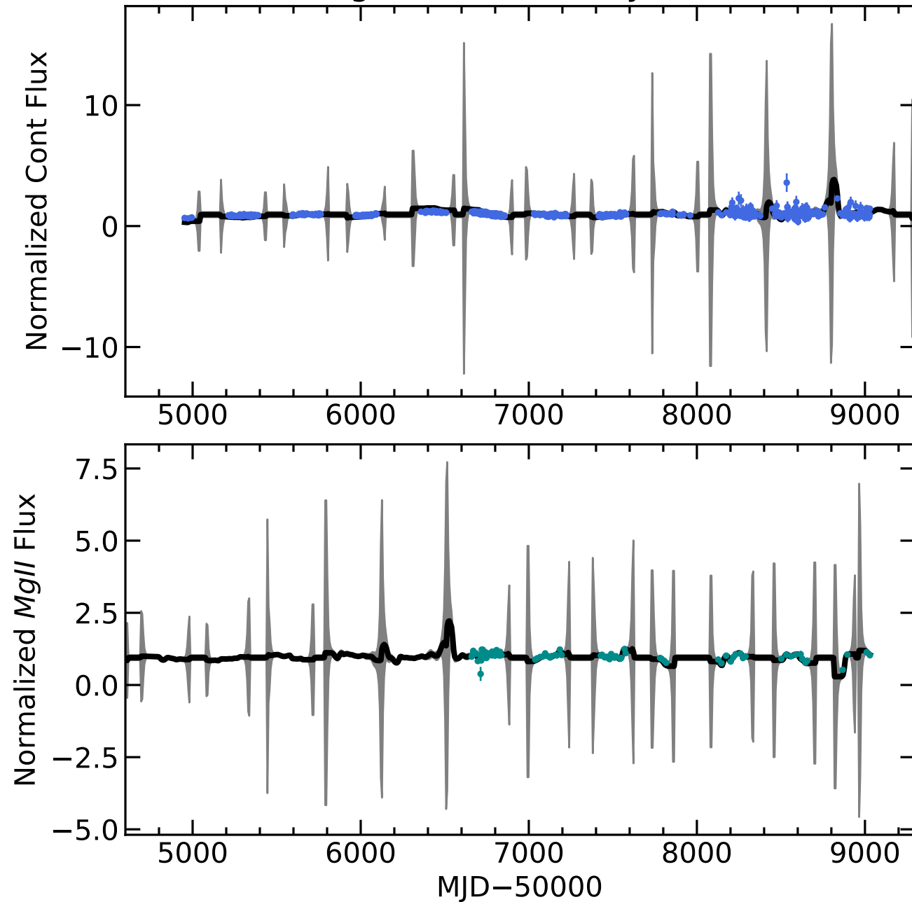
RM064 Light Curves (w/ PyROA model)
