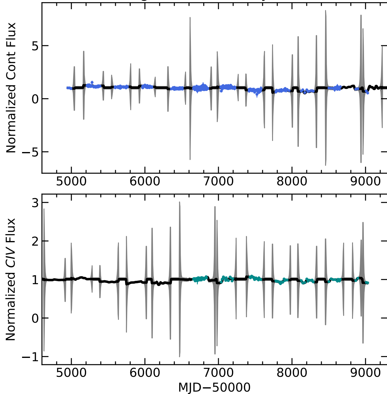
RM065 Light Curves (w/ PyROA model)
