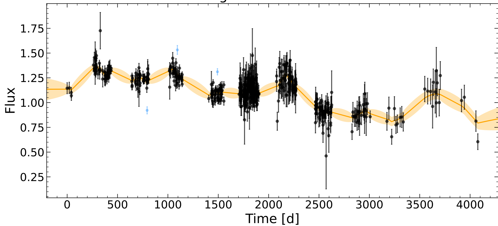
Light Curve of cont
