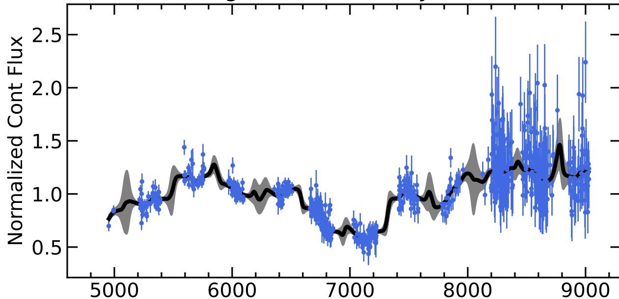
RM066 Light Curves (w/ PyROA model)
