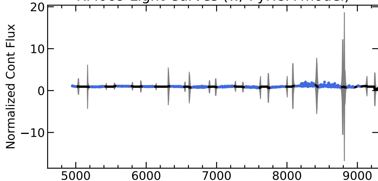
RM069 Light Curves (w/ PyROA model)
