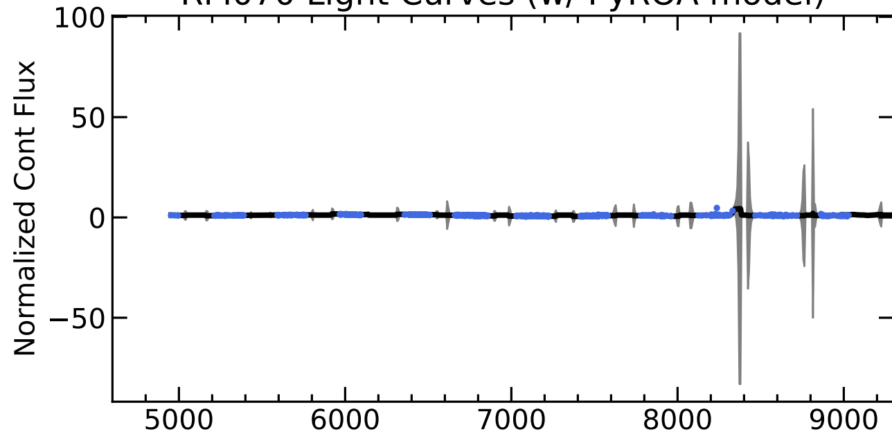
RM070 Light Curves (w/ PyROA model)
